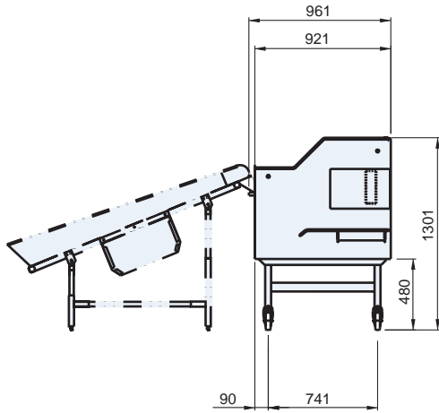
Buffer conveyor, front connection
